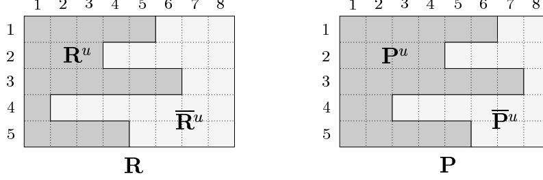
Figure 2: Example division of \mathbf{R} and \mathbf{P} for N = 8 , m = 5 , and \mathbf{u} = (6,4,7,2,5) .
